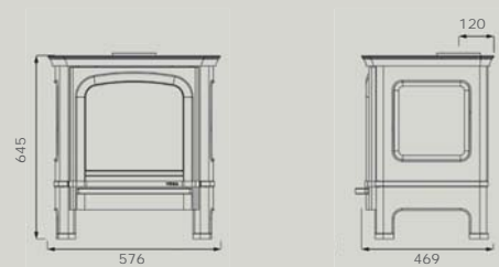
VEGA B7 / C7
